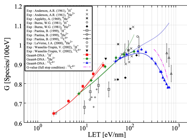
FIG. 2. LET dependence of G-values of \text{H}_2\text{O}_2 by ^1\text{H}^+ (red square), ^4\text{He}^{2+} (green circle), and ^{12}\text{C}^{6+} (blue triangle) ion beams with multiple ionization processes (solid line) and without multiple ionization processes (dotted line) at 1 \mu\text{s} after irradiation. Solid and dotted lines represent the trends obtained by Genat4-DNA simulation with and without the multiple ionization processes, respectively. The G-value of \text{H}_2\text{O}_2 by full stop condition of ^{12}\text{C}^{6+} ion beams with multiple ionization processes is shown with the dashed-dotted magenta line. Experimental data presented by Anderson and Hart, 31 Appleby and Schwarz, 32 Burns and Sims, 33 Pastina and LaVerne, 34 LaVerne et al. , 35 and Vasselin-Trupin et al. 36 are used for comparison with simulated LET dependence of G-values.
