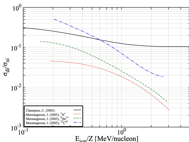
FIG. 1. The ratio of double-to-single ionization cross sections \sigma_{di}/\sigma_{si} for ^1\text{H}^+ (dotted red line), ^4\text{He}^{2+} (dashed green line), and ^{12}\text{C}^{6+} (dashed-dotted blue line) ion beams reported by Meesungnoen and Jay-Gerin. 11 The values of \sigma_{di}/\sigma_{si} reported by Champion 25 for a variety of ions at intermediate velocities and gaseous water are also shown for the sake of comparison (solid black line).
