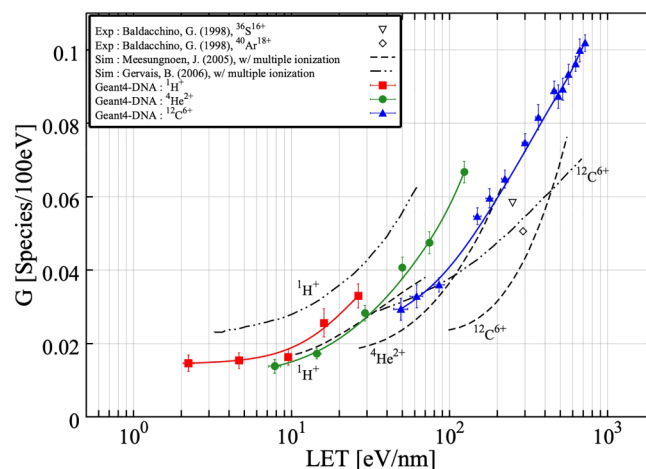
FIG. 3. LET dependence of G-values of \text{HO}_2^\bullet + \text{O}_2^{\bullet-} by ^1\text{H}^+ (red square), ^4\text{He}^{2+} (green circle), and ^{12}\text{C}^{6+} (blue triangle) ion beams with multiple ionization processes (solid line) at 1 \mu\text{s} after irradiation. Solid lines represent the trends obtained by Genat4-DNA simulation with the multiple ionization processes. The dashed and dashed-dotted-dotted black lines represent simulation results with the multiple ionization processes reported by Meesungnoen and Jay-Gerin 11 and Gervais et al. 12 respectively. Sets of experimental data presented by Baldacchino et al. 38,39 were used for comparison with simulated LET dependence of G-values.
